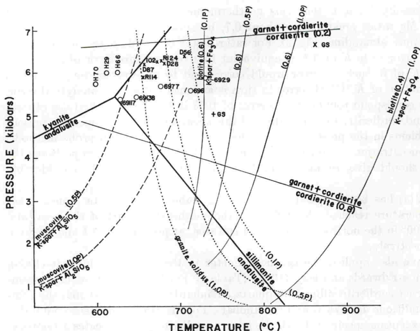
Fig. 3. PT projection of garnet cordierite equilibrium and other relevant experimental data. The figures in brackets on the experimental univariant curves give the Fe/Fe + Mg ratio of the starting materials, while the figures at the end of the curves (e.g. 0.5 P) give the water pressure as a fraction of total pressure. The biotite breakdown curve is calculated for the quartz-fayalite magnetite buffer. Numbered and lettered points are those shown in Tables 1 and 4. The two points labelled GS represent the migmatitic and nonmigmatitic garnet-cordierite gneisses analyzed by Gable and Sim (1969). Specimen 69117 contains andalusite plus sillimanite, while all others contain sillimanite, although specimens H 70, H 29, and H 66 appear to fall in the Kyanite field
